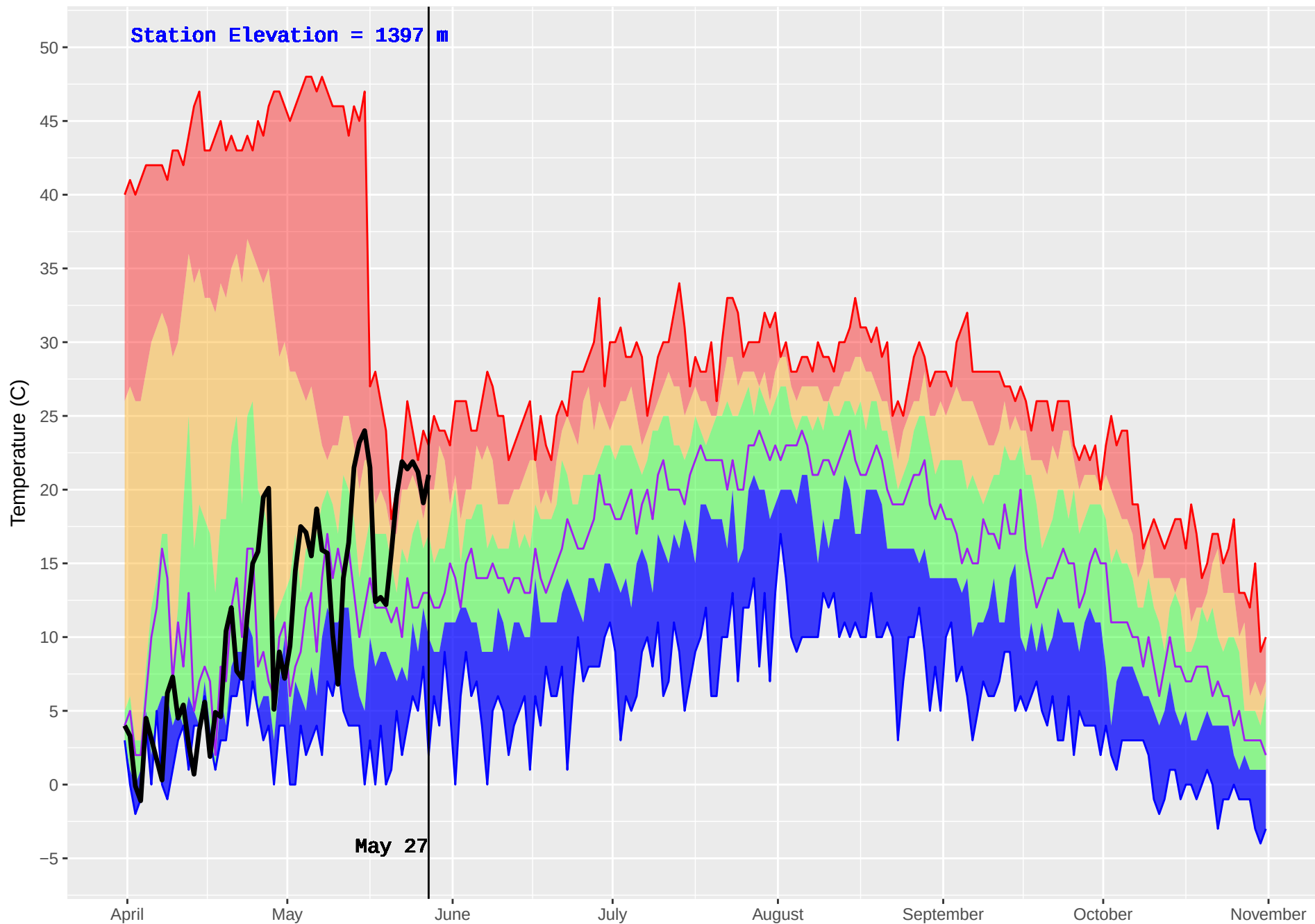
NANCY GREEN (407) : Historical (1992–2016) and Current (2018) Noon Temperature
