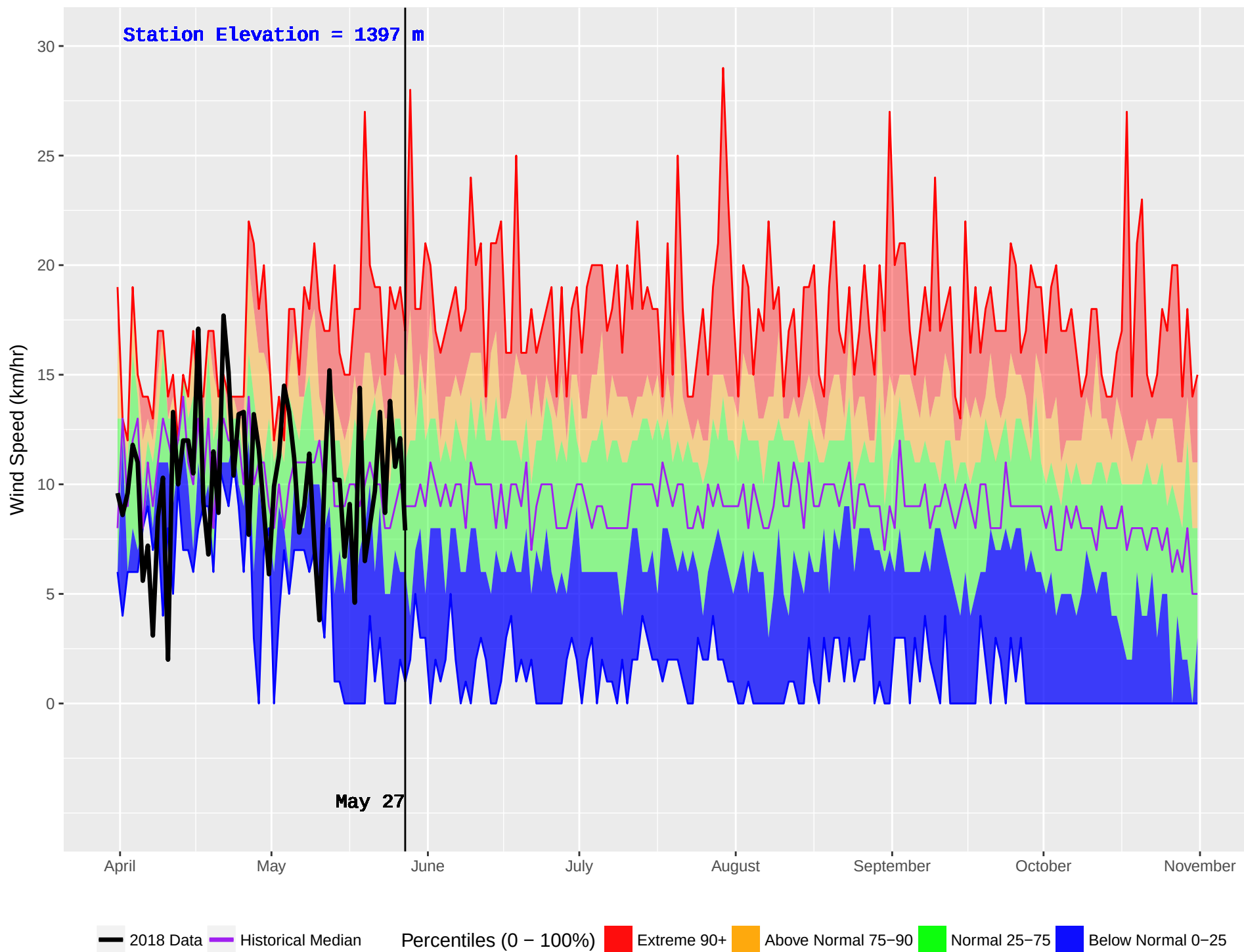
NANCY GREEN (407) : Historical (1992–2016) and Current (2018) Noon Wind Speed
