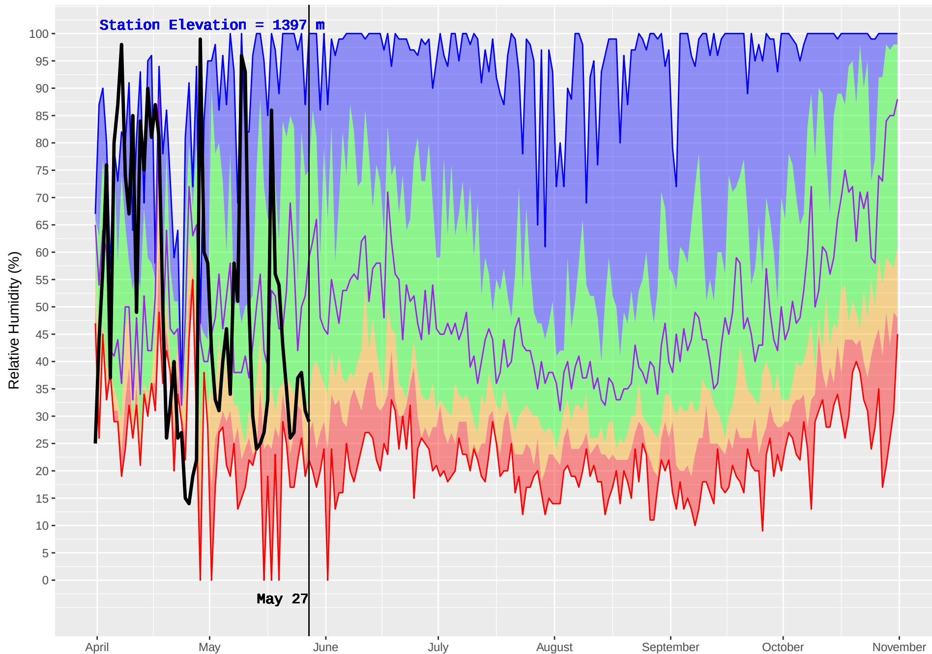
NANCY GREEN (407) : Historical (1992–2016) and Current (2018) Noon Relative Humidity
