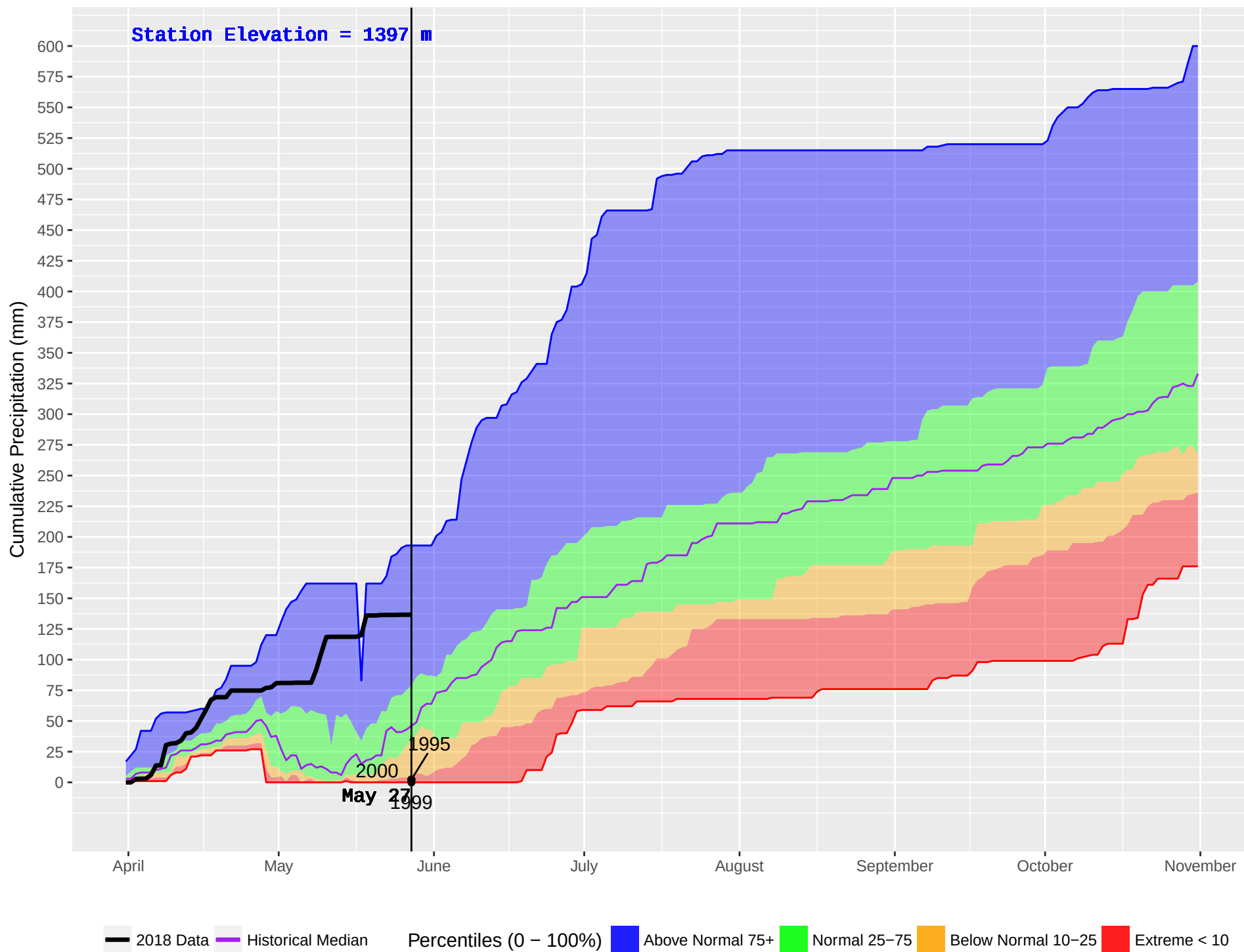
NANCY GREEN (407) : Historical (1992–2016) and Current (2018) Noon Cumulative Precipitation
